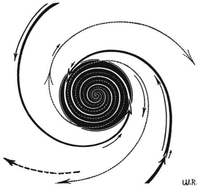
FIG. 73. This same principle, as demonstrated in Figs. 71-72 is also demonstrated by the atomic and nebular systems, which form where two anodes are united by collision. This figure demonstrates the one-way of motion which produces both effects of life and death in Nature.
