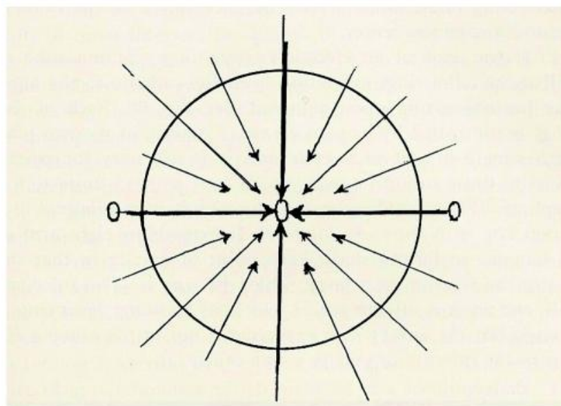
FIG. 59. Illustrating the radial universe concept.
