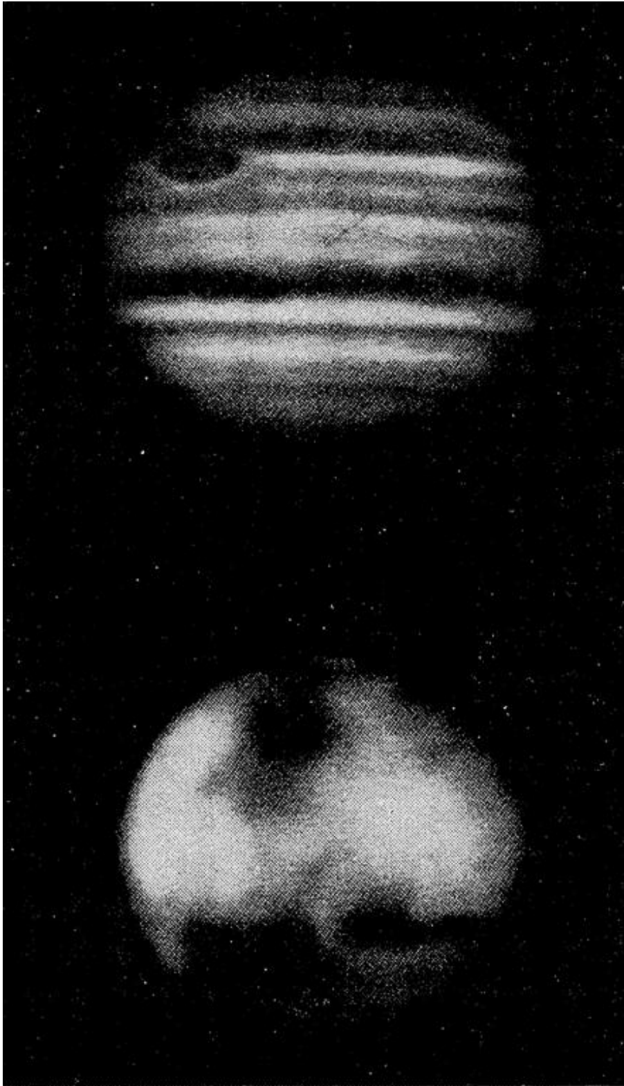
FIG. 3. JUPITER and MARS.
