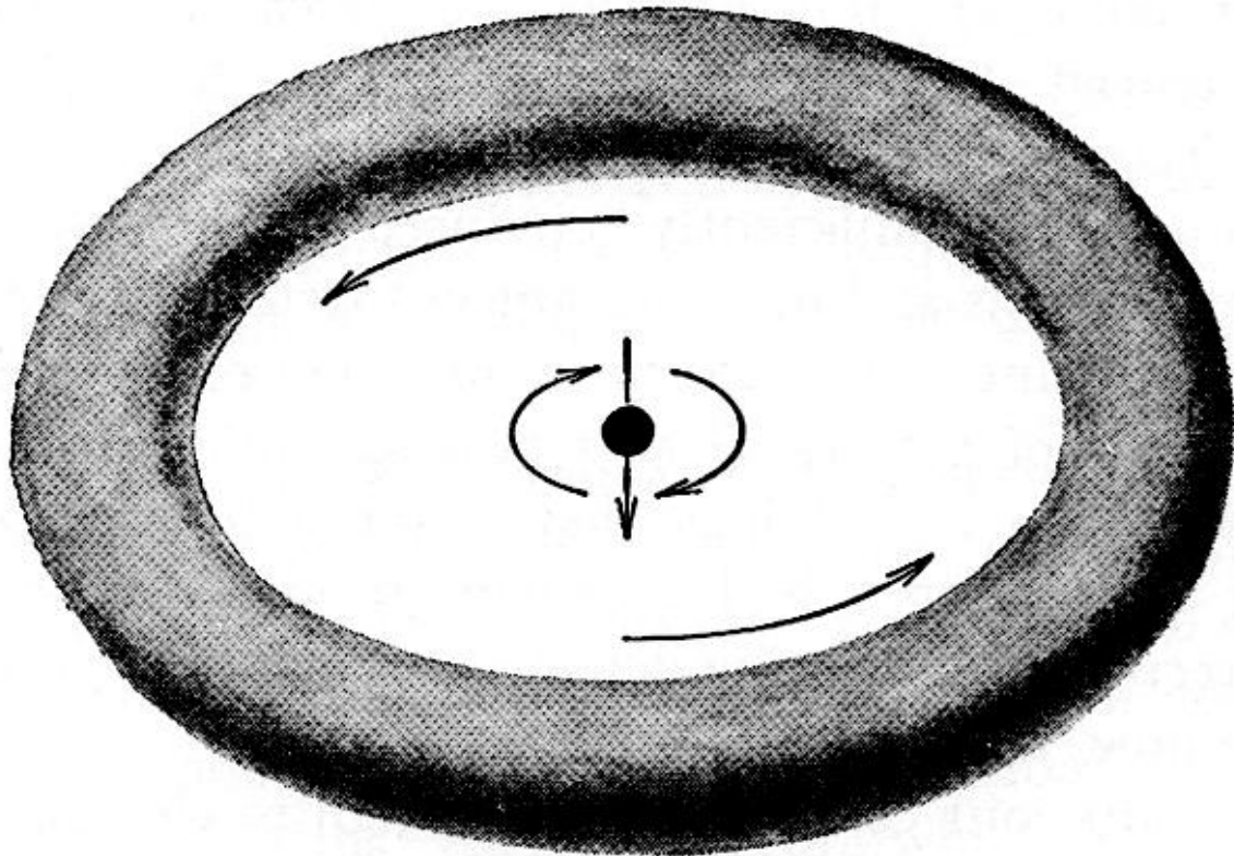
FIG. 35. "MESON THEORY suggests that the proton may actually consist of a spinning 'bare nucleon' which is essentially a point, surrounded part of the time by a rotating meson cloud."
