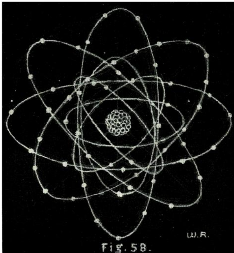
The Rutherford-Bohr atom.
