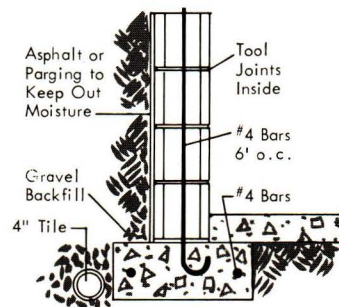
EXTERIOR WALL
